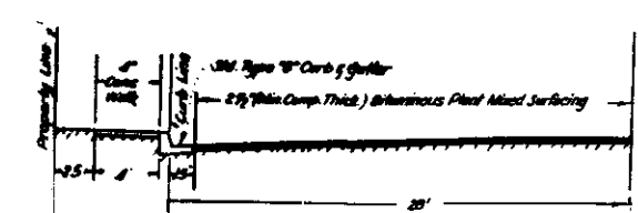
TYPICAL SECTION 37TH STREET SCALE 1"=6'
